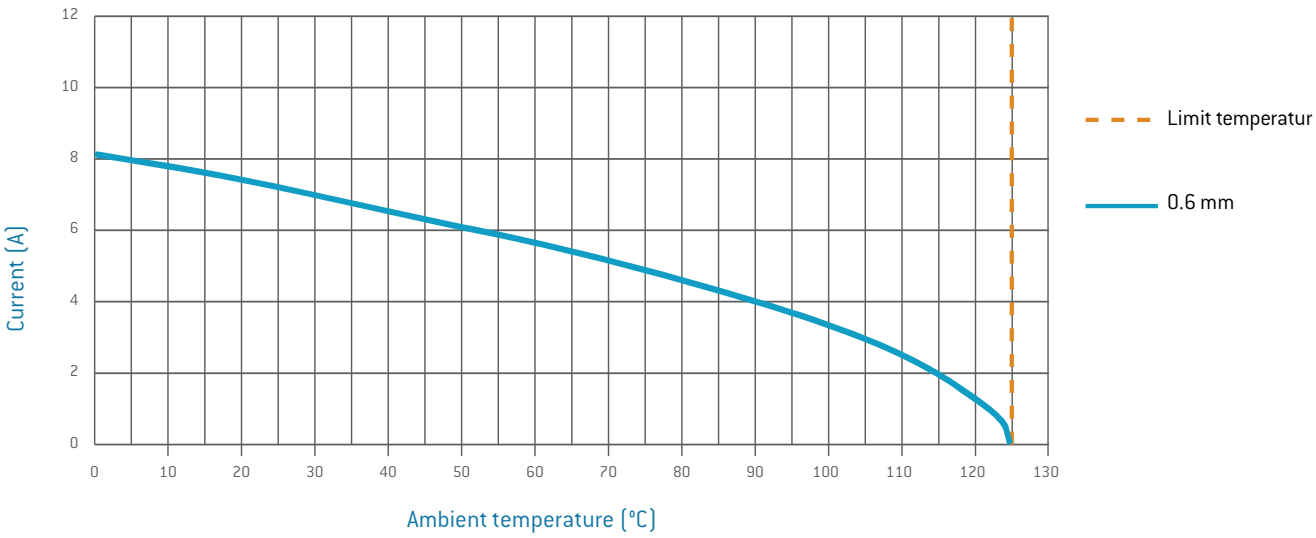
NOMINAL SINGLE CONTACT CURRENT LOAD FOR SPRING LOAD CONTACT (PISTON DIAMETER 0.6 mm)
