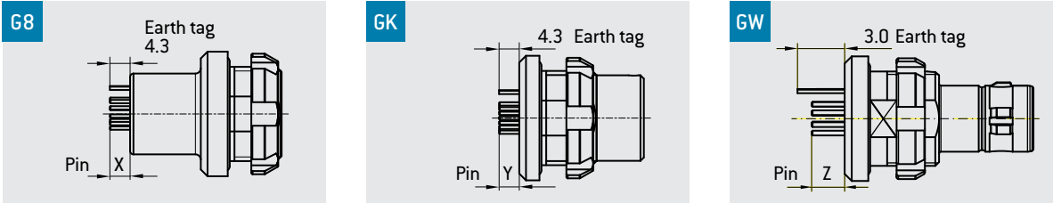
LENGTH EARTH TAG AND PIN
